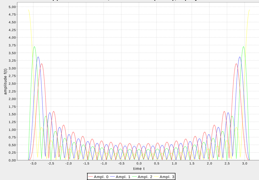
Dropped Dimensions, time domain (norm), 4 polynomials
