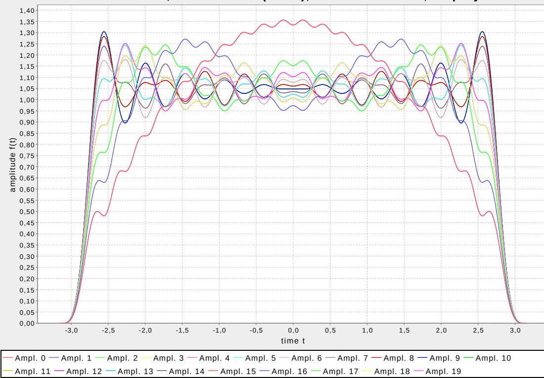
Advanced PCC-OFDM, time domain (norm), 24 carriers used, 20 polynomials
