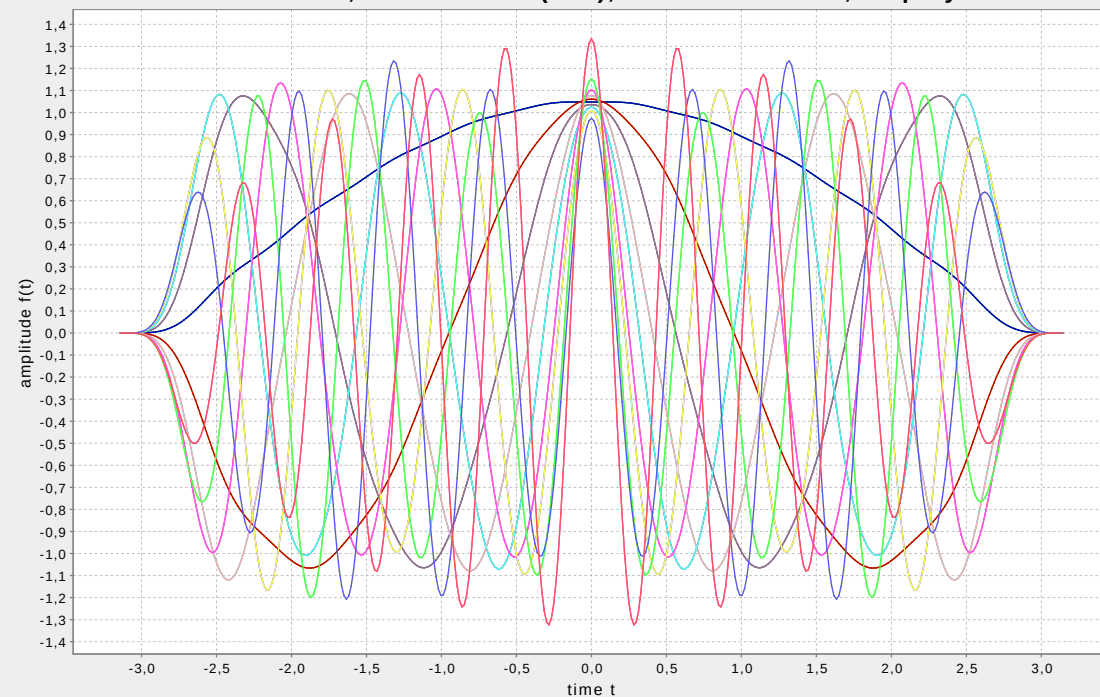
Advanced PCC-OFDM, time domain (cos), 24 carriers used, 20 polynomials
