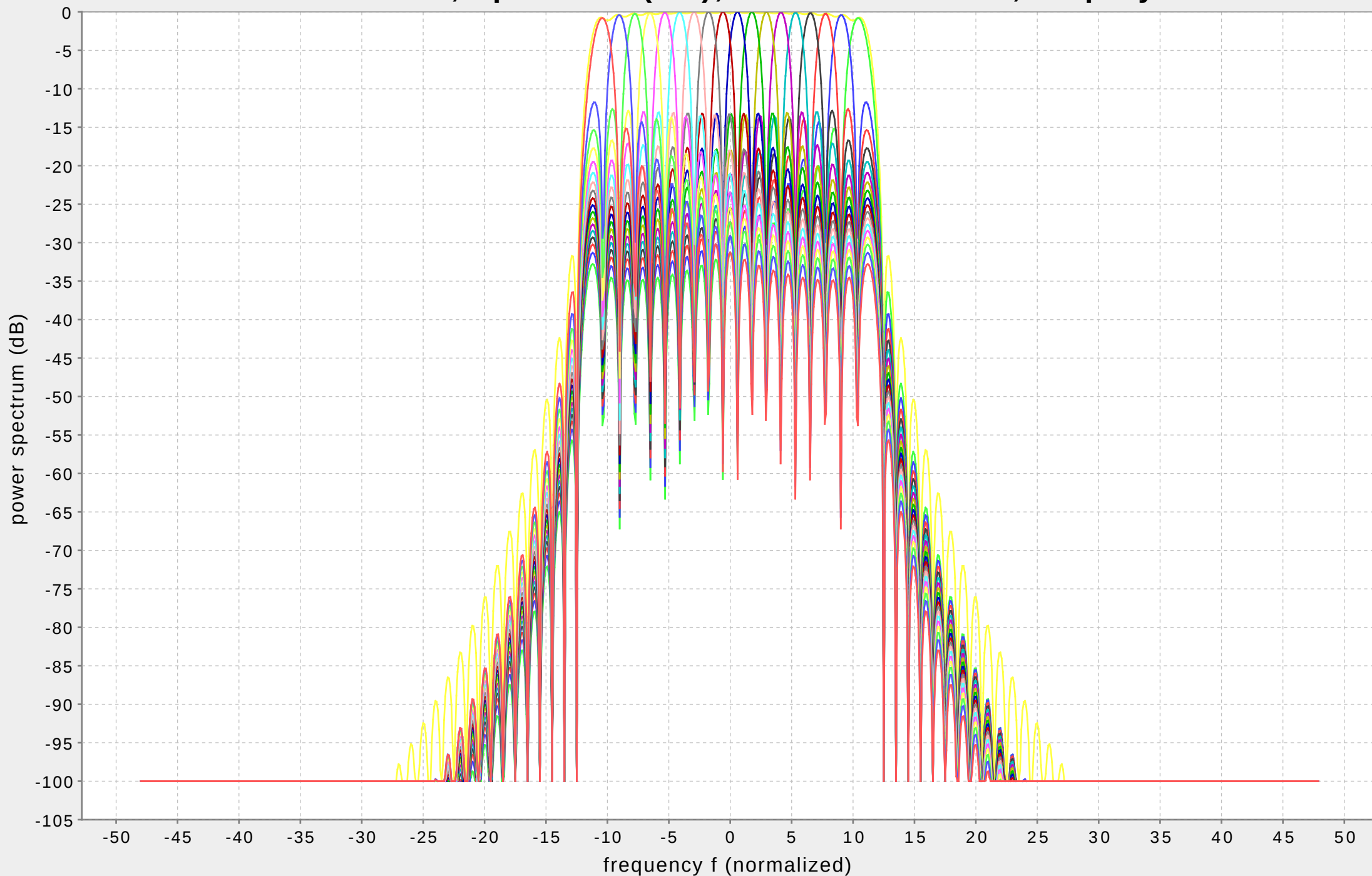
Advanced PCC-OFDM, spectrum (far), 24 carriers used, 18 polynomials
