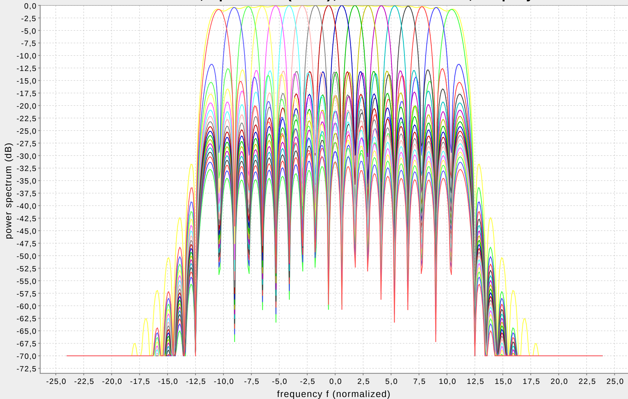
Advanced PCC-OFDM, spectrum (near), 24 carriers used, 18 polynomials
