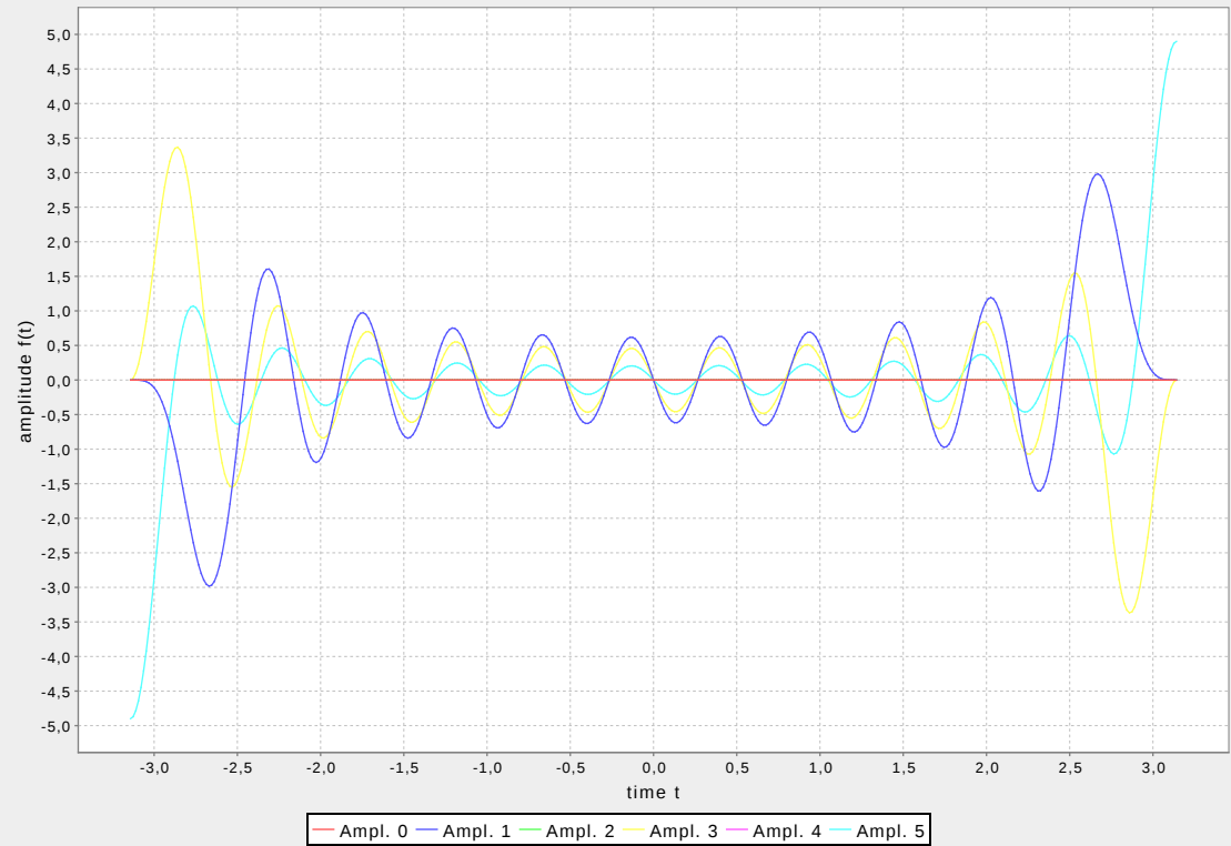
Dropped Dimensions, time domain (sin), 6 polynomials
