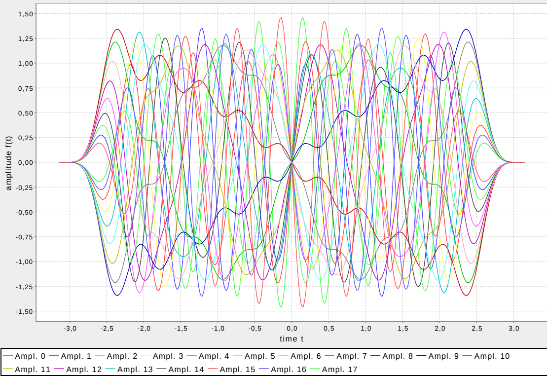
Advanced PCC-OFDM, time domain (sin), 24 carriers used, 18 polynomials
