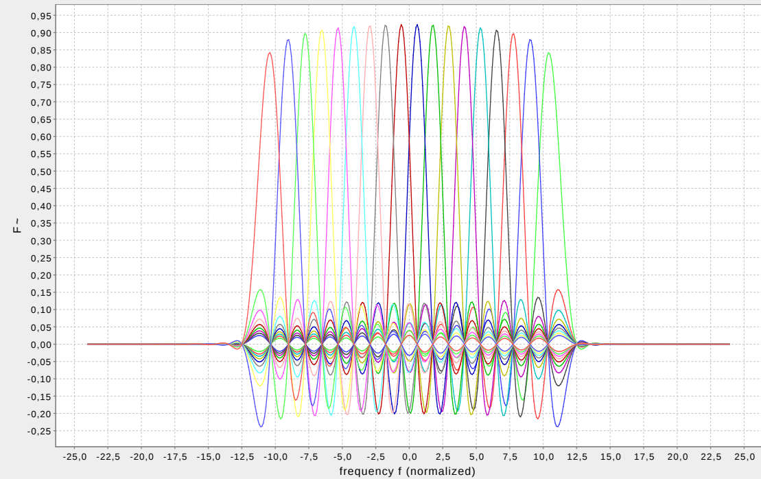
Advanced PCC-OFDM, frequency domain, 24 carriers used, 18 polynomials
