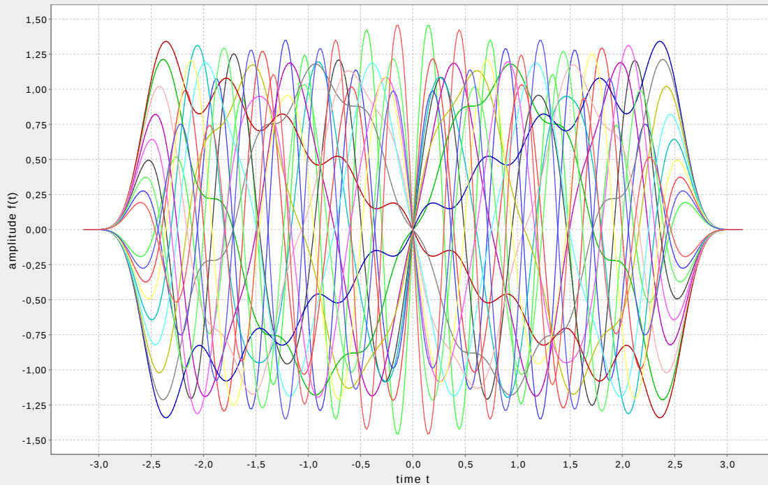
Advanced PCC-OFDM, time domain (sin), 24 carriers used, 18 polynomials
