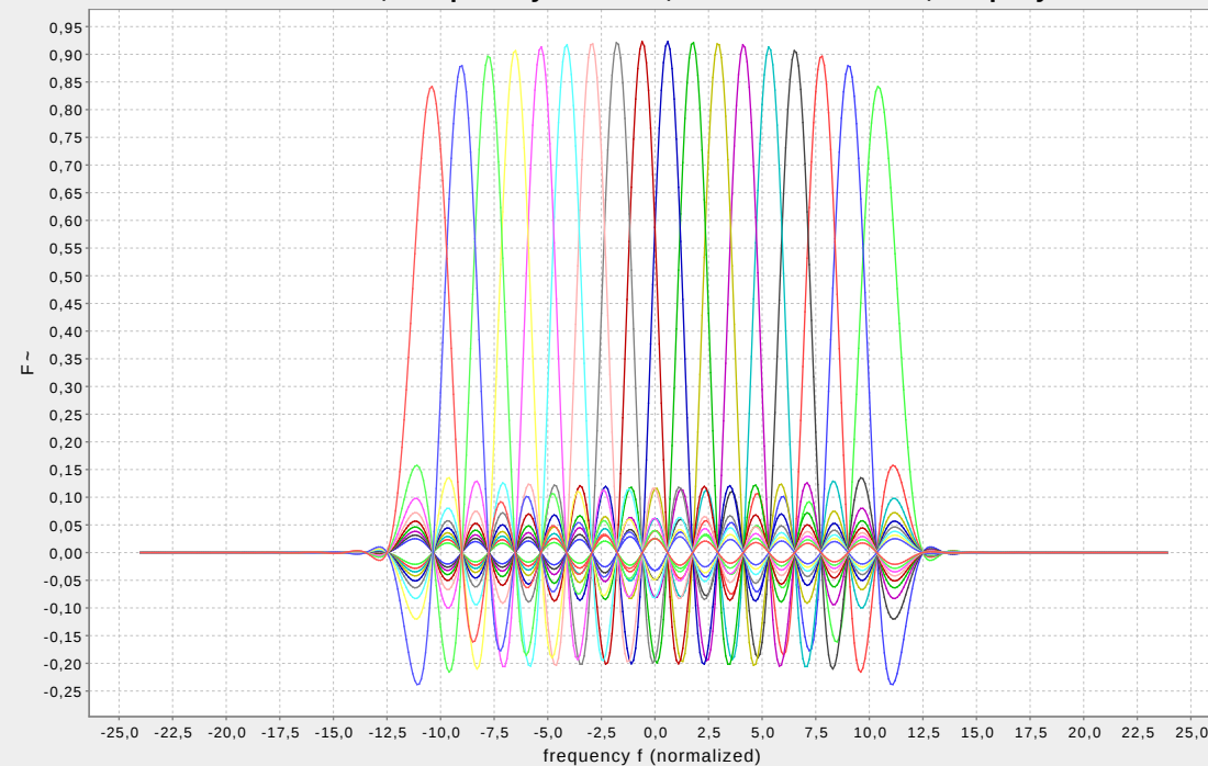
Advanced PCC-OFDM, frequency domain, 24 carriers used, 18 polynomials
