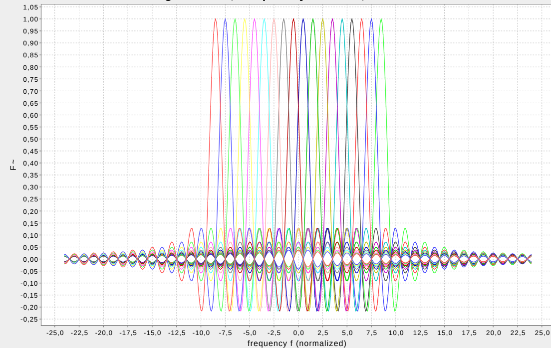
Rectangle-OFDM, frequency domain, 18 carriers
