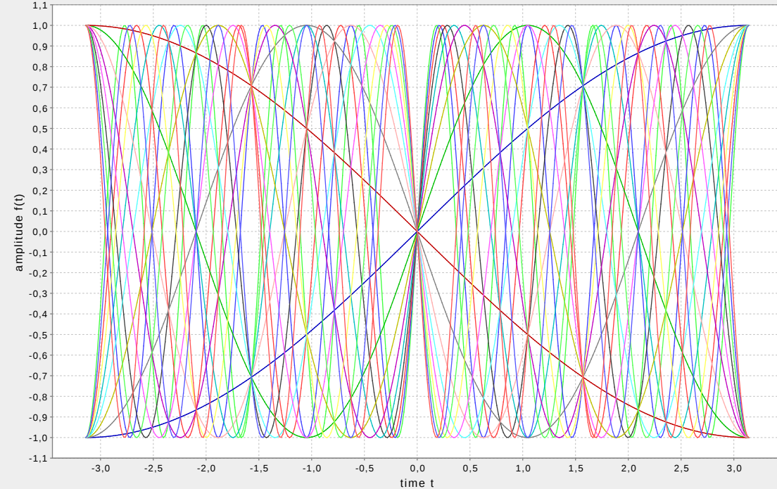
Rectangle-OFDM, time domain (sin), 18 carriers
