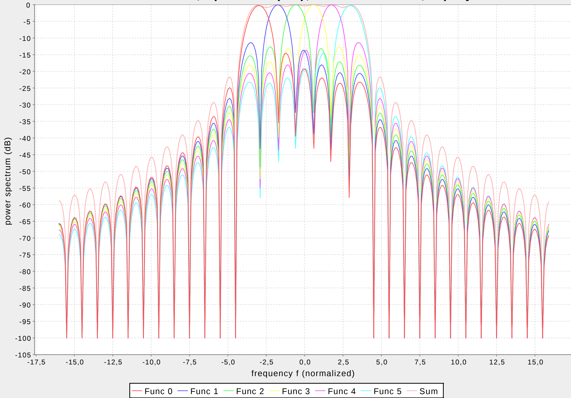
Advanced PCC-OFDM, spectrum (far), 8 carriers used, 6 polynomials
