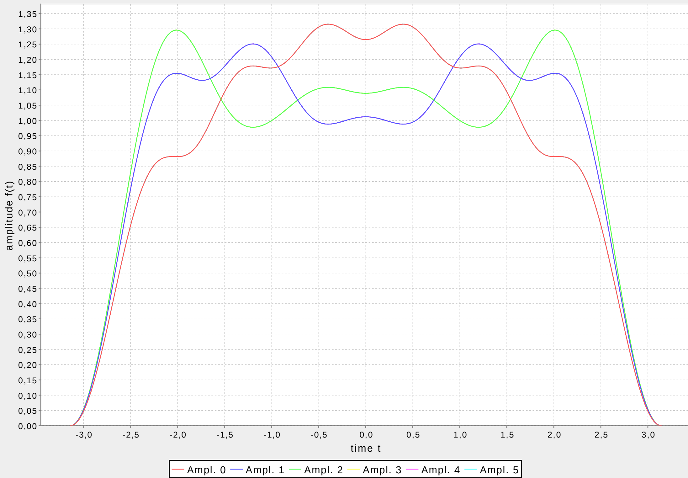
Advanced PCC-OFDM, time domain (norm), 8 carriers used, 6 polynomials
