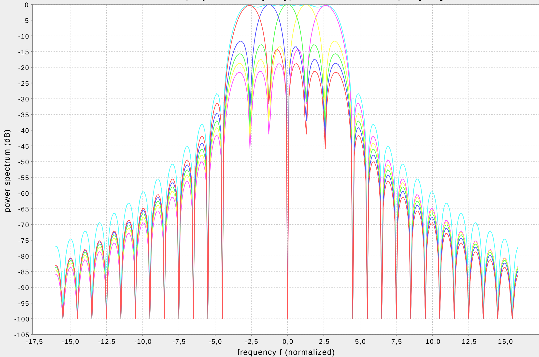
Advanced PCC-OFDM, spectrum (far), 8 carriers used, 5 polynomials
