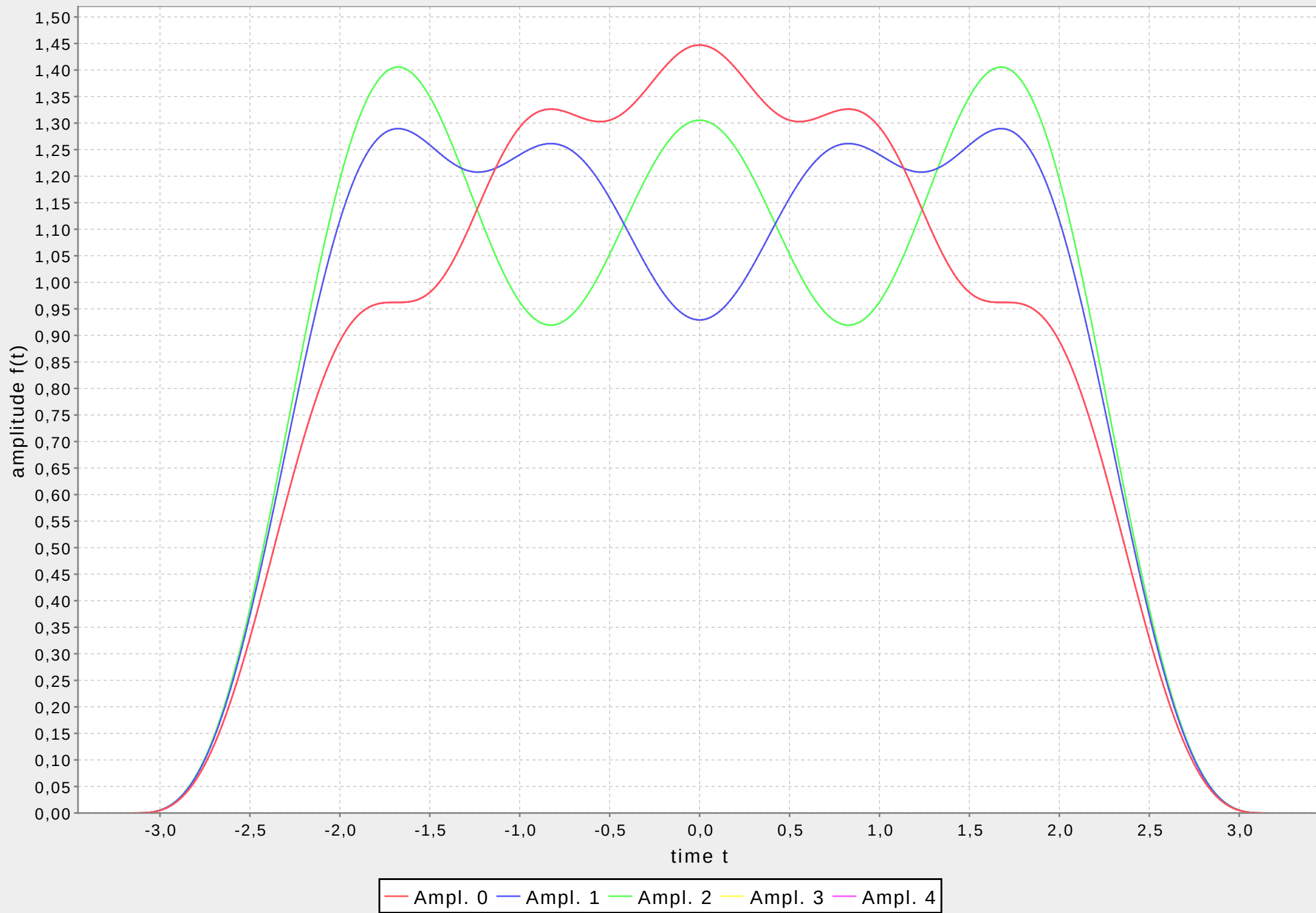
Advanced PCC-OFDM, time domain (norm), 8 carriers used, 5 polynomials
